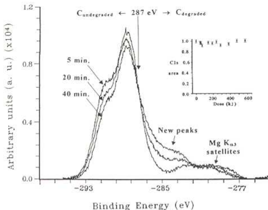
Figure 2 Typical C1s spectra of Teflon AF1600 (power source = 200 W), and C1s total area versus X-ray dose. Inset: C1s peak area as a function of X-ray dose.
