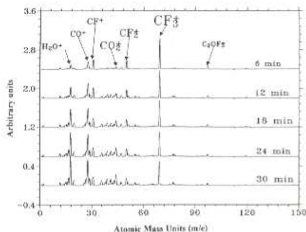
Figure 5 Mass spectra of fragments produced on exposure of Teflon AF1600 to X-rays at a source power of 120 W. The background spectrum, at t = 0 , has been subtracted.
