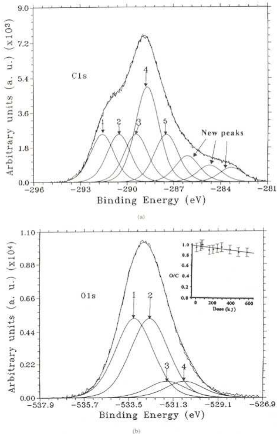
Figure 3 Peak separation of (a) C1s, (b) O1s, and (c) F1s spectra of Teflon AF1600 subsequent to a radiation dose of 200 W/40 min; O/C and F/C versus dose; the ratios are normalized to maximal values. Insets to (b) and (c): O/C and F/C ratios, respectively, as a function of X-ray dose.
