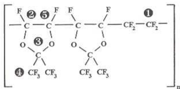
Figure 1 The structure of the Teflon AF1600 repeat unit.
